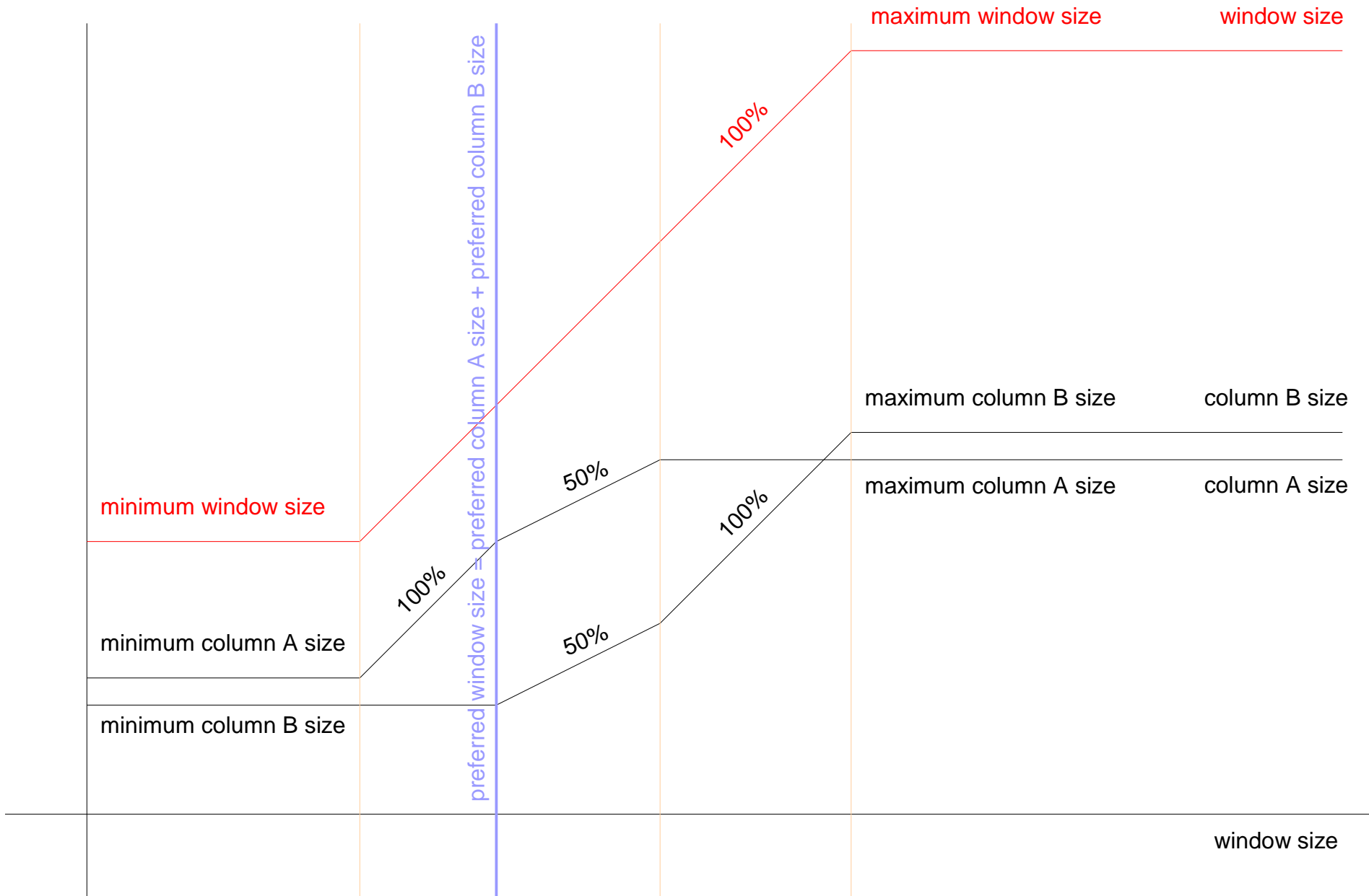
column size calculation algorithm
